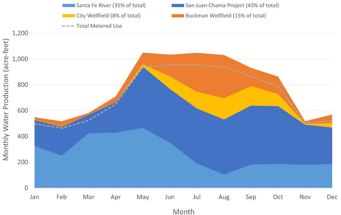
6 – Monthly Potable Water Production by Source and Use, 2024
