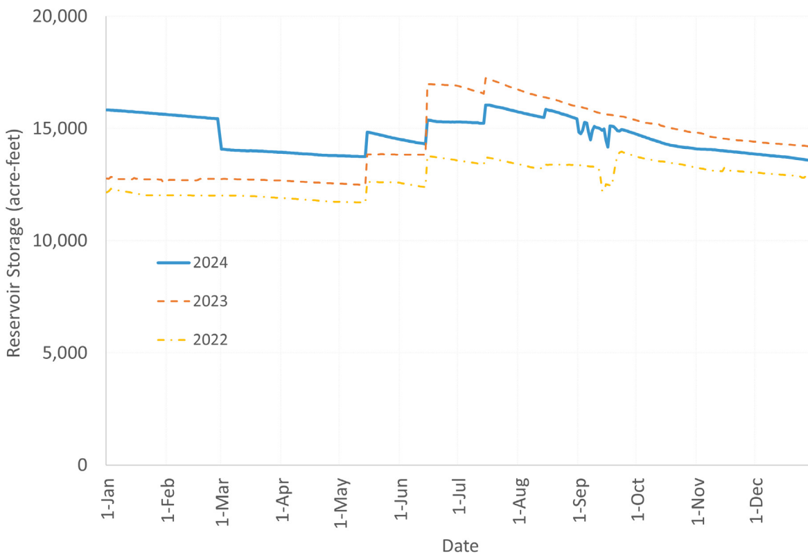
Total San Juan-Chama Project Storage
