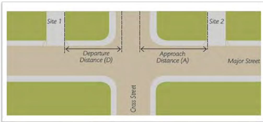
Figure 47: Driveway Distance from Intersection, Approach and Departure
