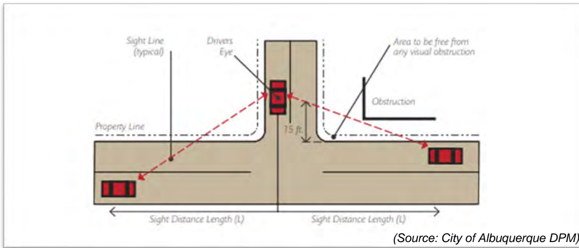
Figure 50: Intersection Sight Distance Criteria
