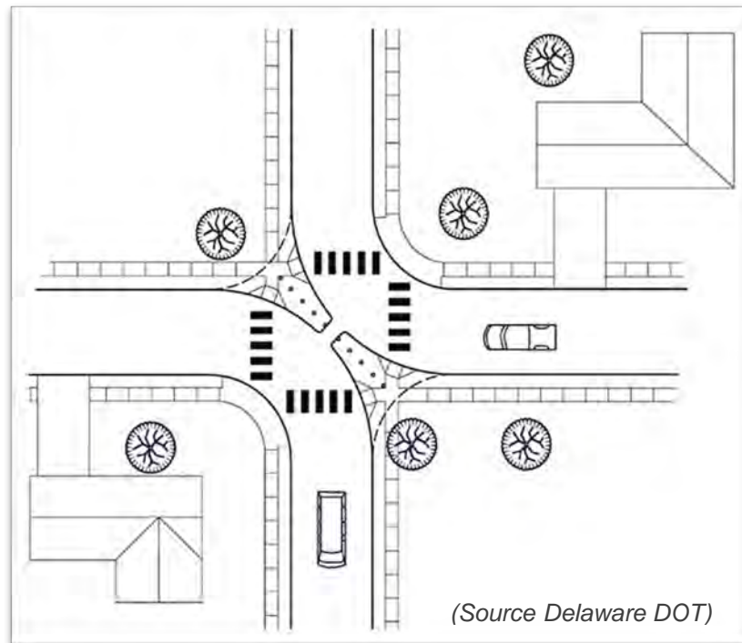
Figure 60: Diagonal Diverter Schematic
