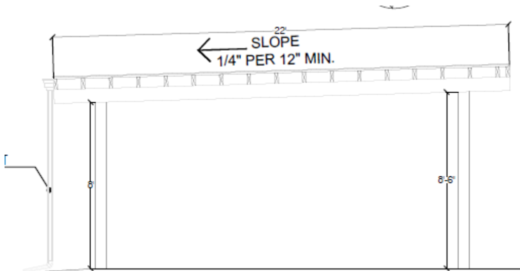
Figure 4: Elevation of the Visible Side of the Carport
