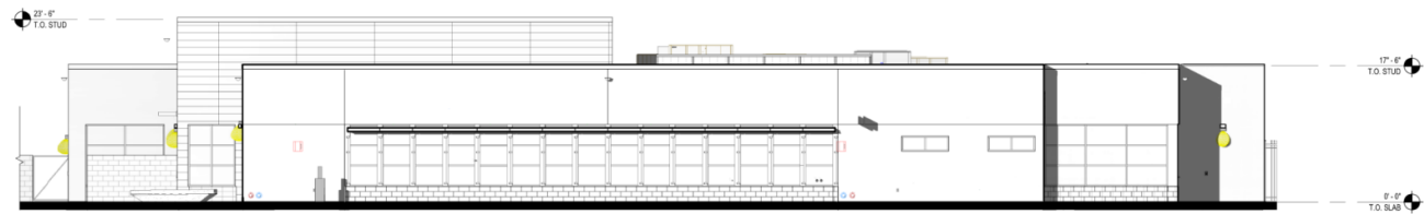
A1 OPERATIONS BUILDING - SOUTH ELEVATION 18'x14'
