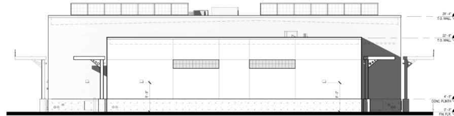
C1 MAINTENANCE FACILITY WEST ELEVATION 1/8" = 1'-0"
