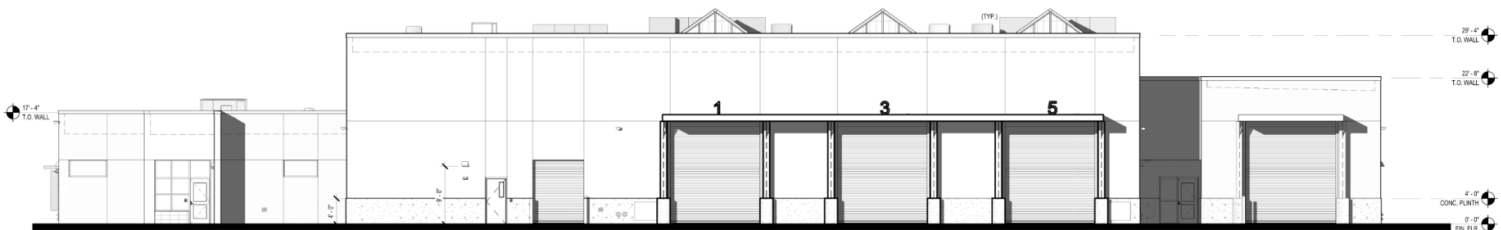
A1 MAINTENANCE FACILITY NORTH ELEVATION 1/8" = 1'-0"
