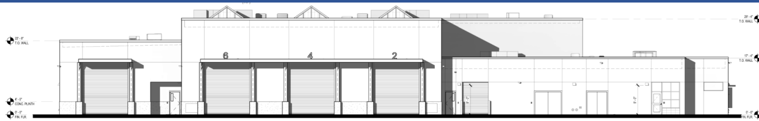
D1 MAINTENANCE FACILITY NEW SOUTH ELEVATION 1/8" = 1'-0"
