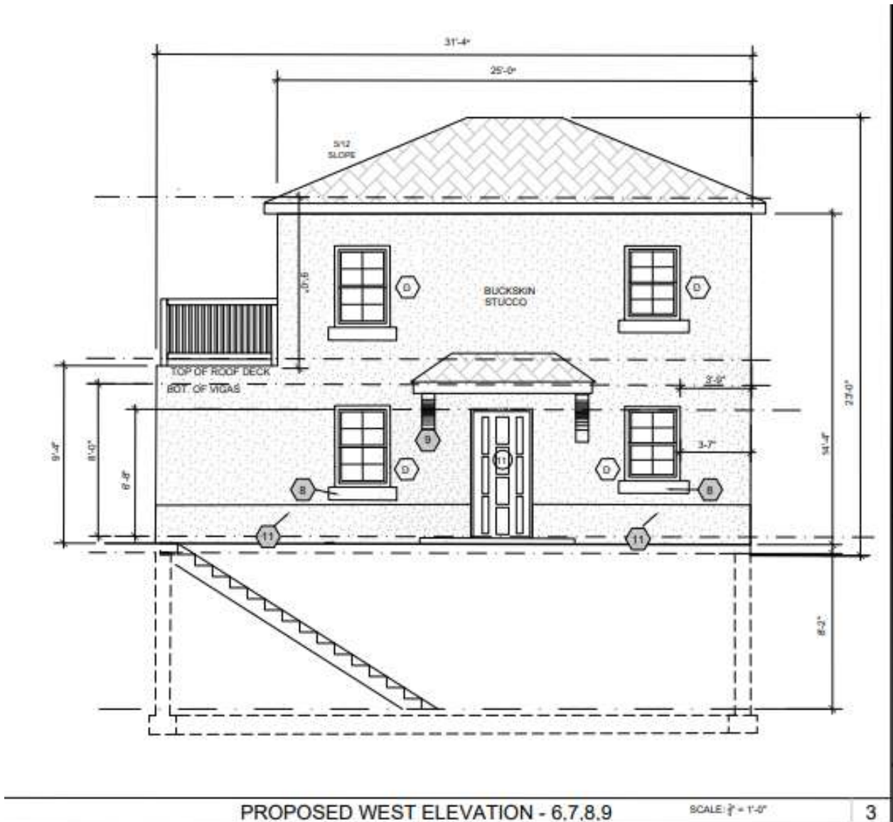
Figure 7. Proposed 219 A Washington Ave West Elevation.
