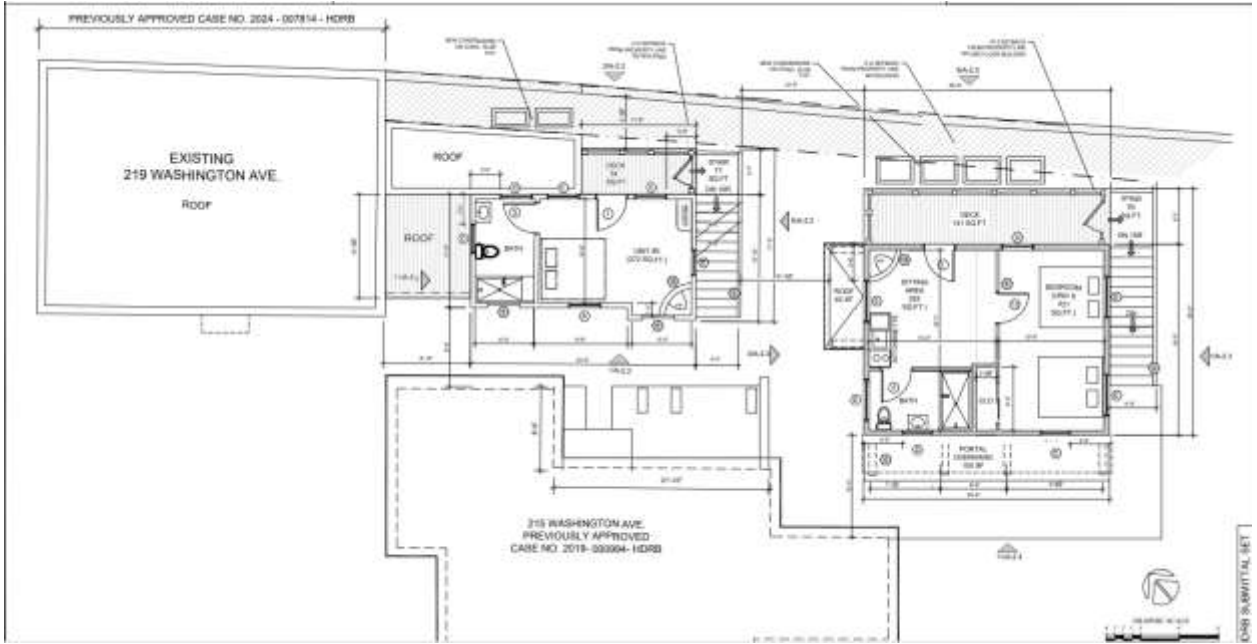
Figure 3. Proposed Second Floor Plan.
