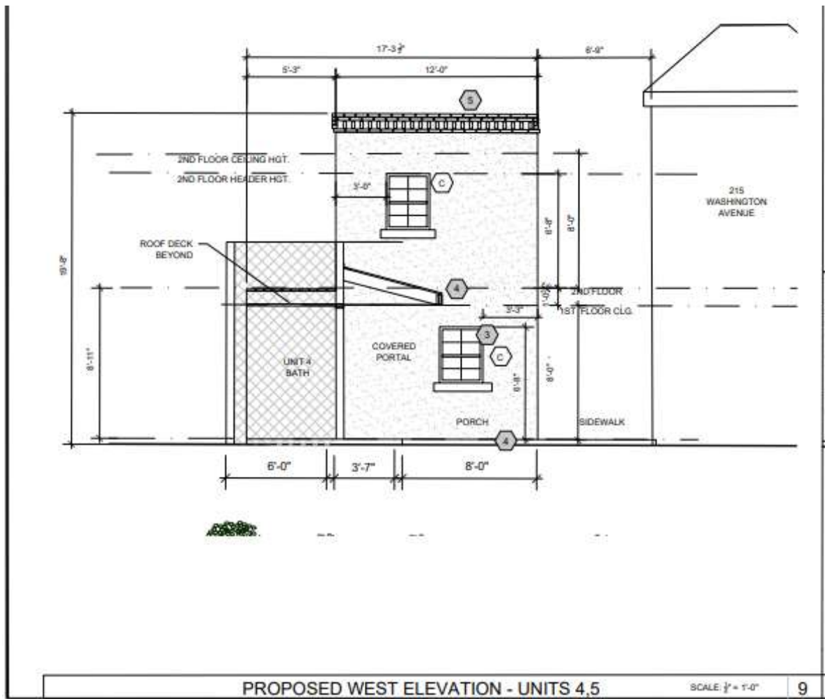
Figure 5. Proposed 219 Washington Ave West Elevation.
