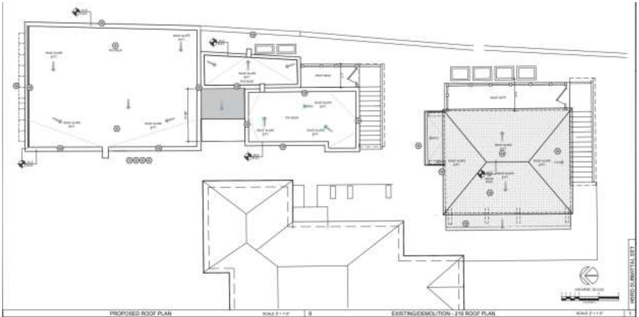
Figure 4. Proposed Roof Plan.
