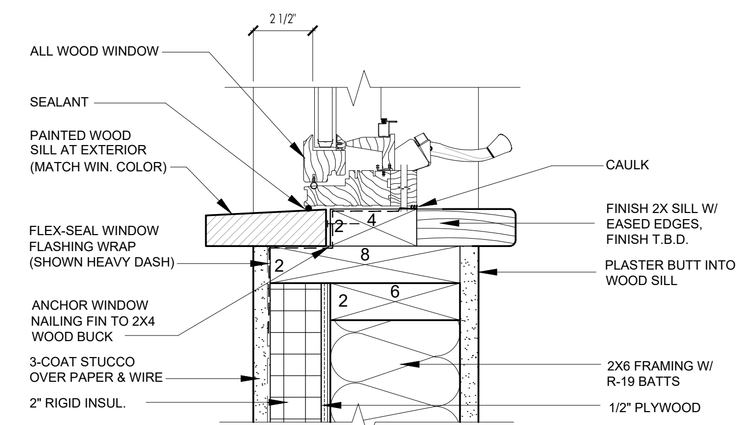
SILL
