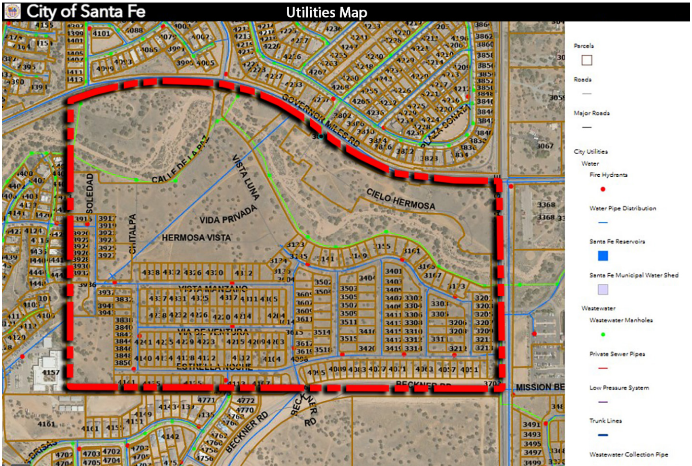
Figure 10 - Utility Map for Overall Subdivision
