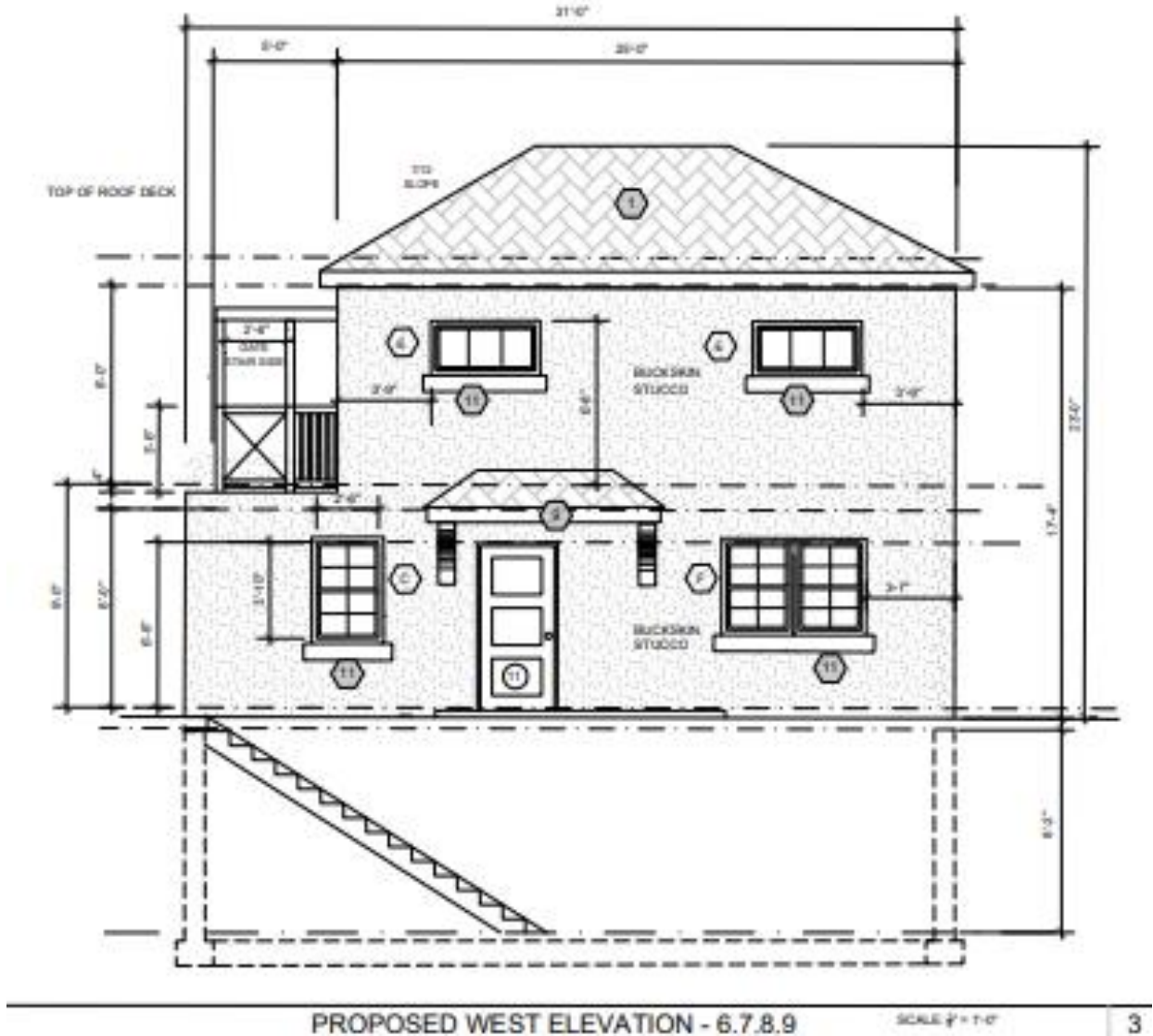
Figure 3. 219A Washington Ave proposed new construction street facing façade.
