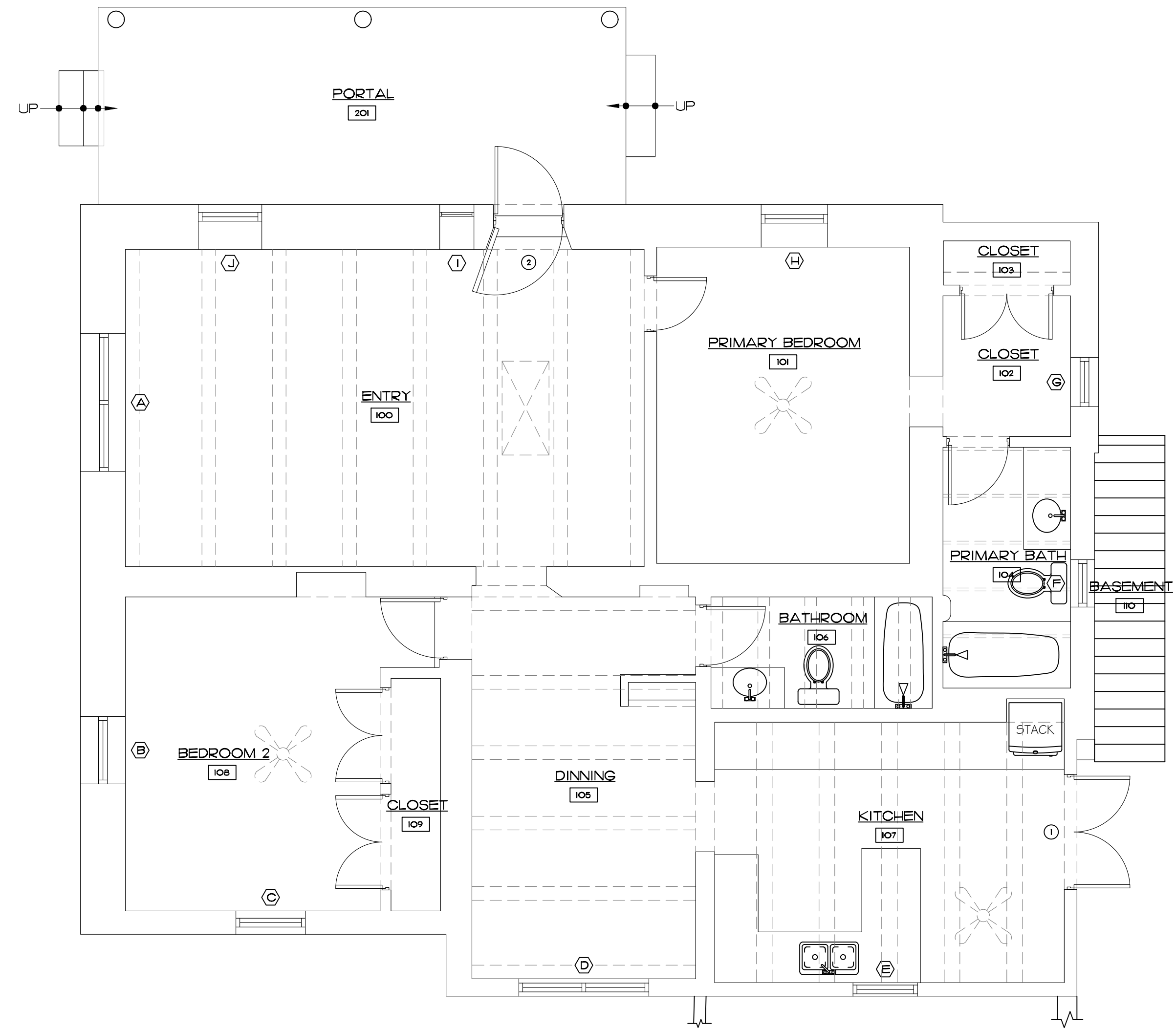
1 A-3.0 EXISTING FLOOR PLAN SCALE: 1/4" = 1'-0"
