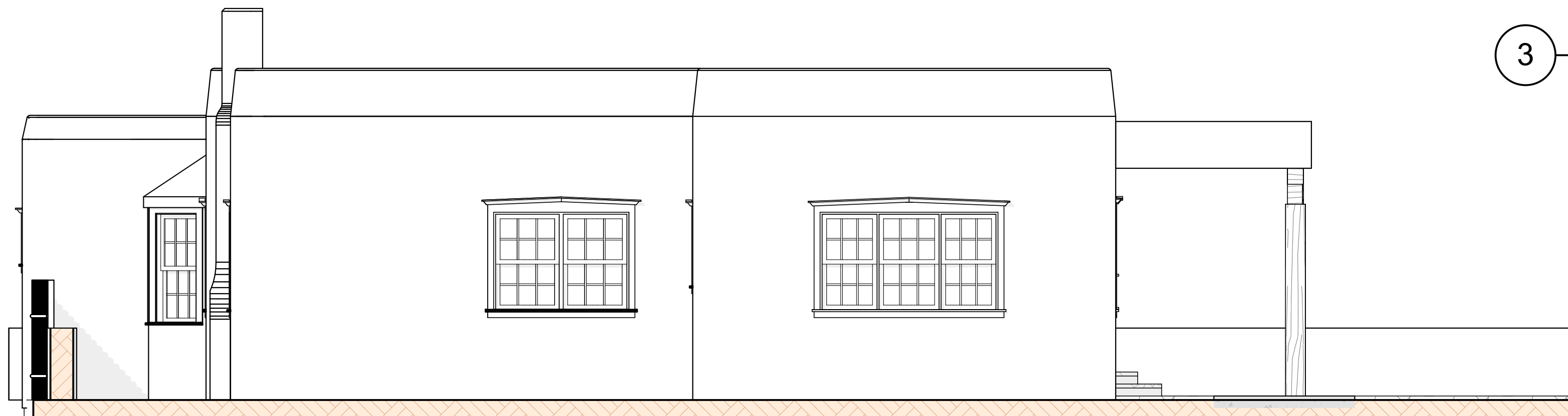
4 Existing West Elevation
