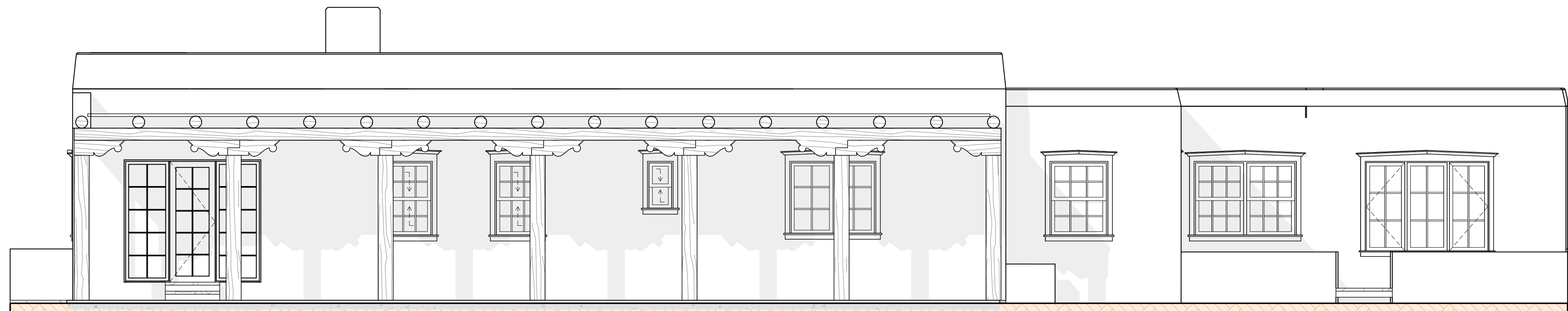
3 Existing South Elevation SCALE: 1/4" = 1'-0"
