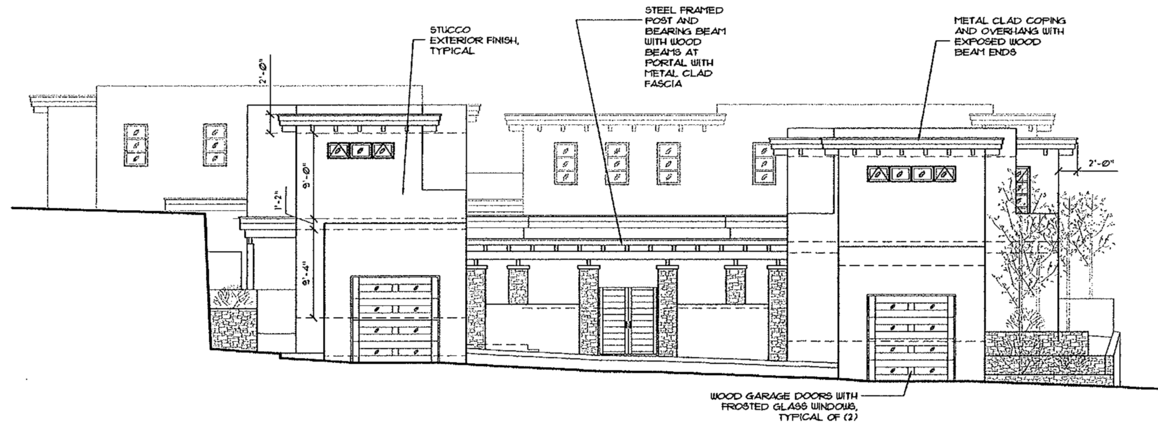
WEST ELEVATION PREVIOUS
